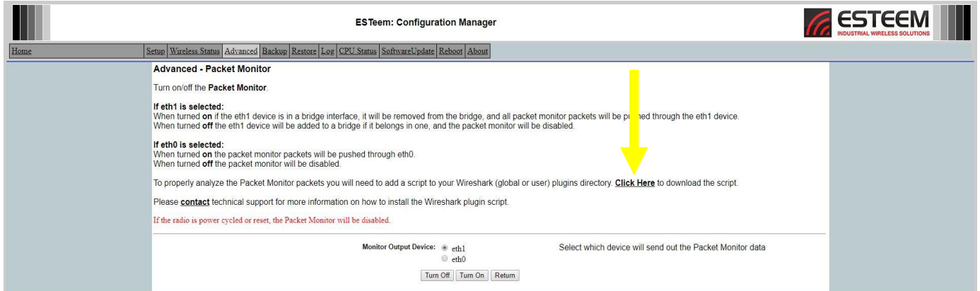
Figure 3: Wireshark Plugin
