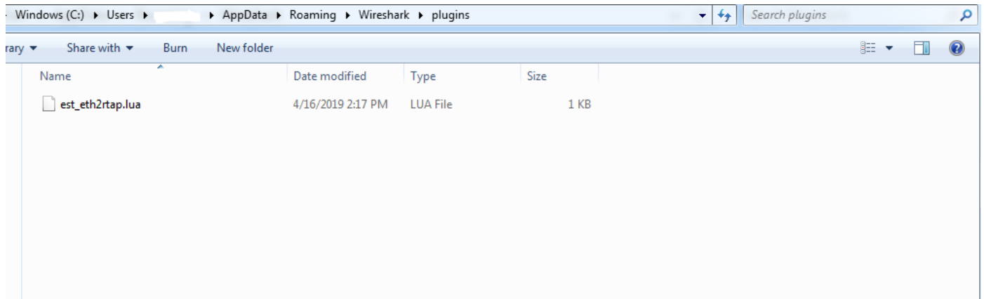
Figure 5: WireShark directory
